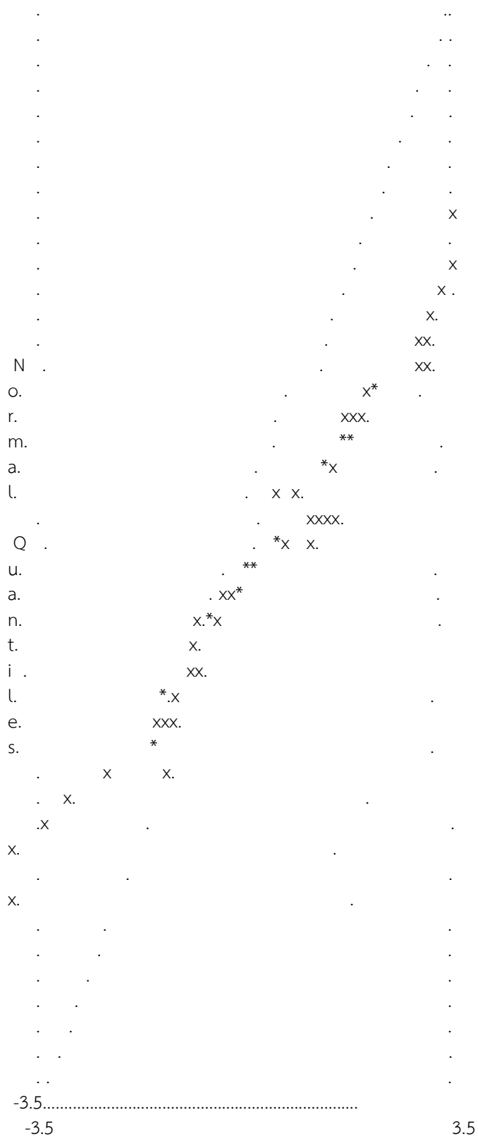
Qplot of Standardized Residuals
